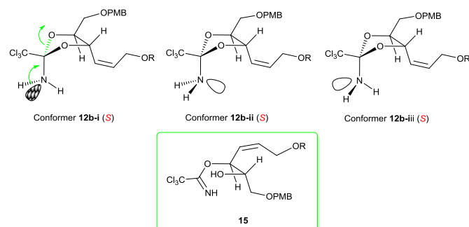
Fig. 11 Only one favorable overlap for most probable staggered conformers of 12b .
