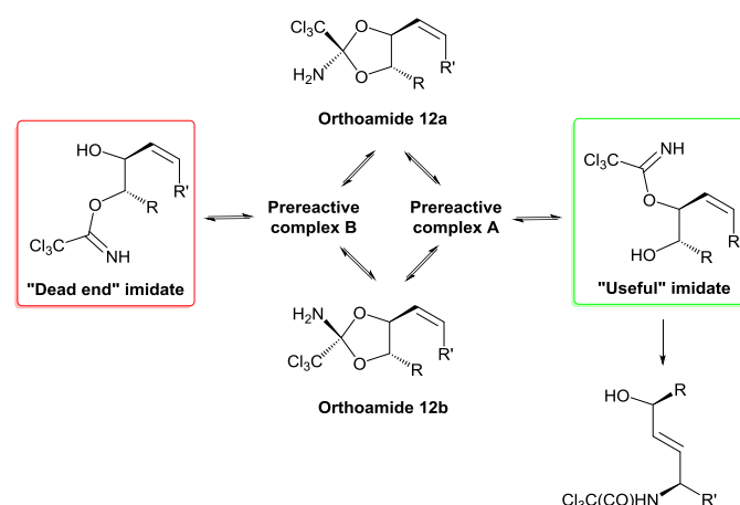
Fig. 12 Species and transformations in the Overman process.
