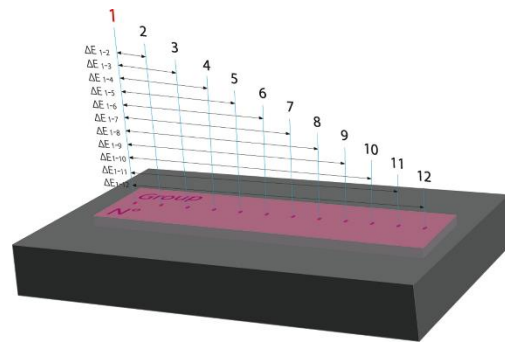
Figure 1. Evaluation of \Delta E in accordance with the acceptability threshold determined by Ren et al. [47]. The sample was placed on a black silicon mold for repositioning. The first measurement was defined as the sample color standard. From this standard point, eleven measurements were taken every 0.5 mm and were each compared to the standard point to determine \Delta E .
