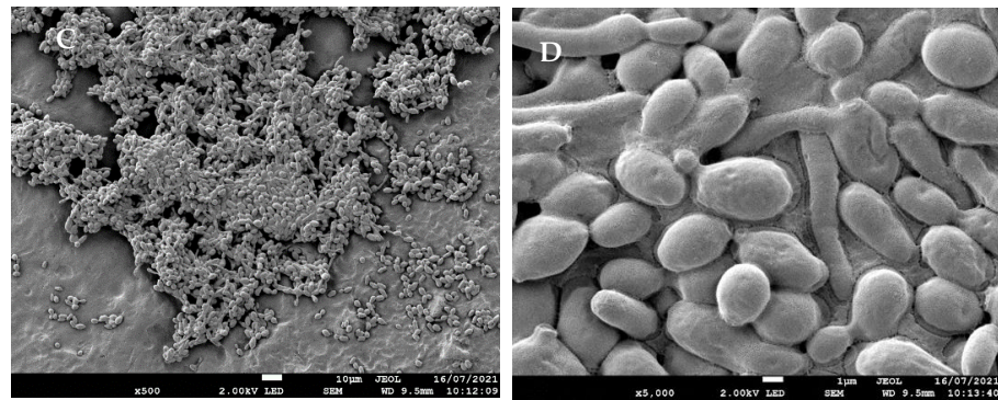
Figure 3. Scanning electron microscopic (SEM) images of C. albicans on glass and resin samples before O 2 NTP treatment. (A) C. albicans repartition on glass slide (G × 100; scale bar = 100 μm); (B) C. albicans repartition on resin sample (G × 100; scale bar = 10 μm); (C) C. albicans clusters on resin sample (G × 500; scale bar = 10 μm); (D) Blastospores, pseudohyphae and hyphae at the top of the clusters were embedded in extracellular polymeric matrix (G × 5000; scale bar = 1 μm).
